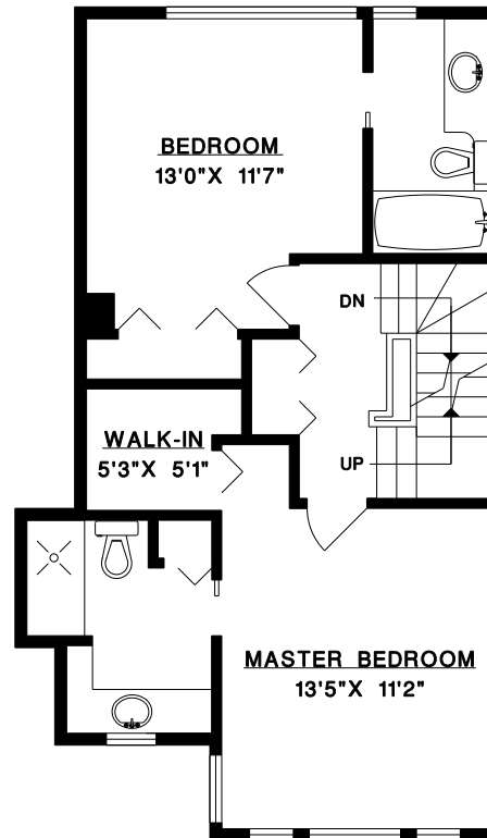
UPPER FLOOR
