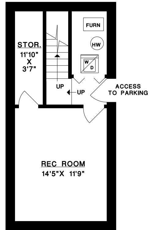
LOWER FLOOR
